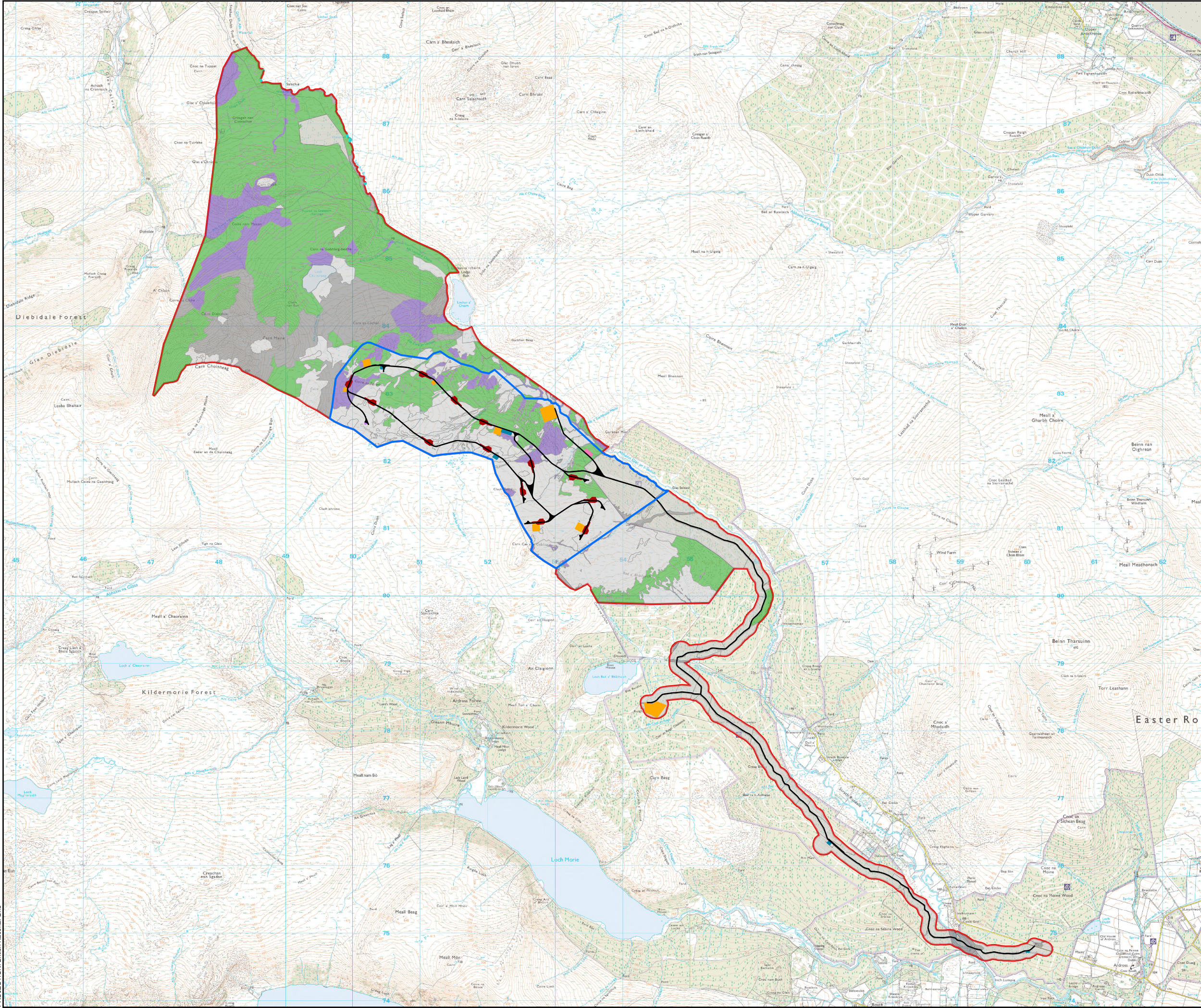
Figure 8.3 Groundwater-dependent Terrestrial Ecosystems Creachan Wind Farm
